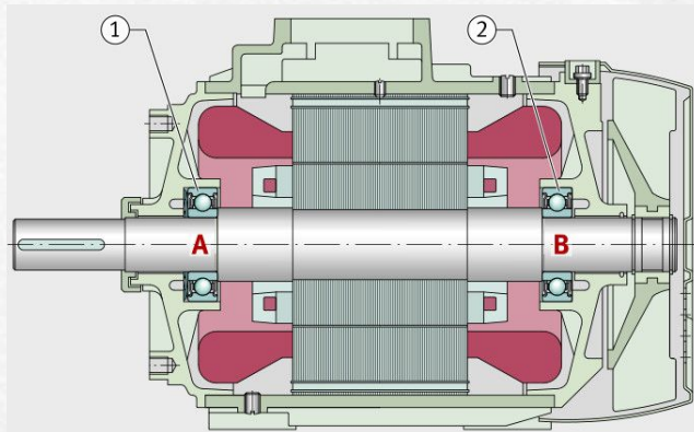
Insulated DGBB in electric motor
