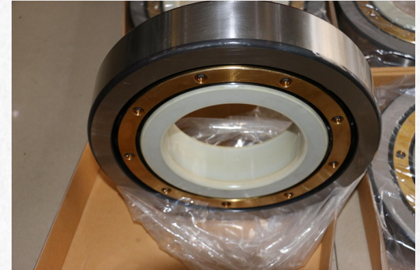
Insulated Deep Groove Ball Bearing (Insulation on inner ring, VL2071)
