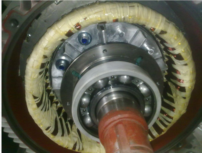
Insulated DGBB in electric motor
